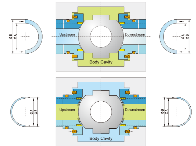
STANDARD SINGLE PISTON EFFECT ( SELF-RELIEVING SEATS )
